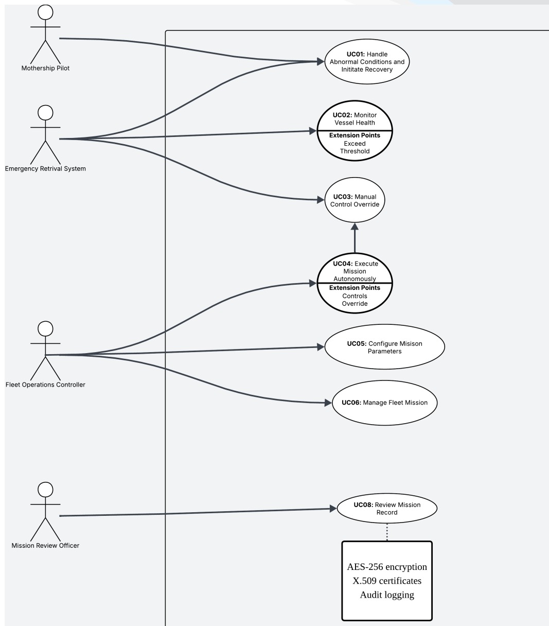
Figure 1: Current lightweight use case view used for this report
